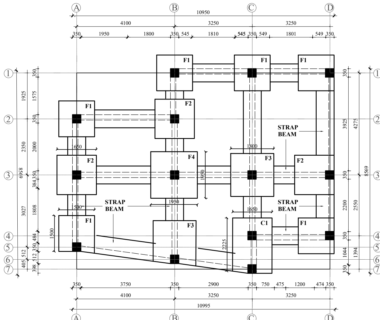
FOUNDATION & TRENCH PLAN SCALE :- 1" = 8'-0"
