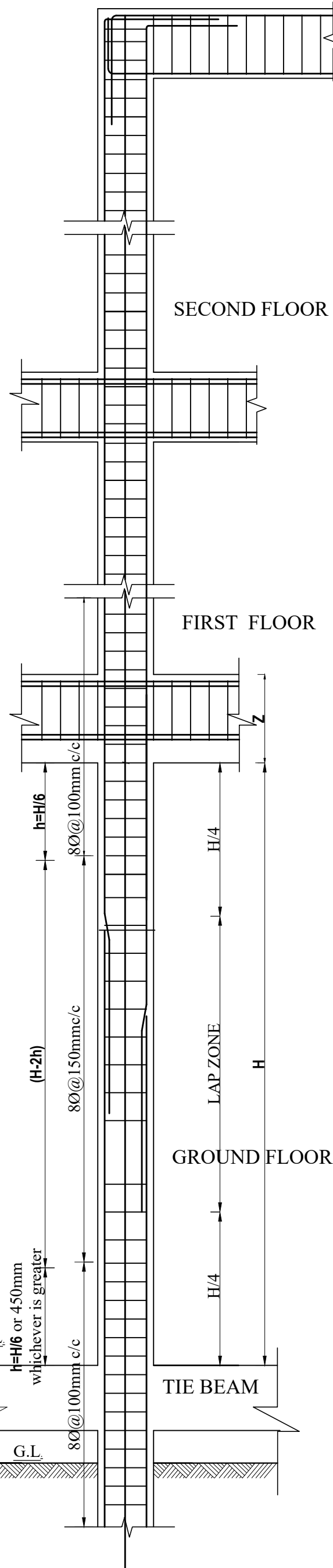
LONGITUDINAL SECTION OF TYPICAL COLUMN SCALE-1/2"=1'-0"
