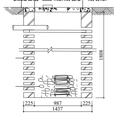
CROSS SECTION OF SOAK PIT SCALE :- 1" = 4'-0"
