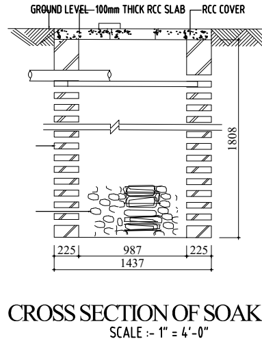
CROSS SECTION OF SOAK PIT SCALE :- 1" = 4'-0"
