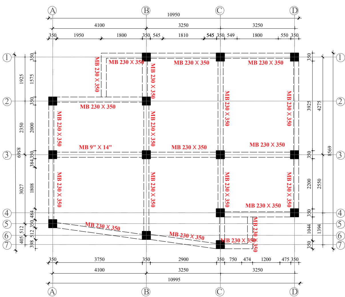
FLOOR BEAM PLAN SCALE :- 1" = 8'-0"
