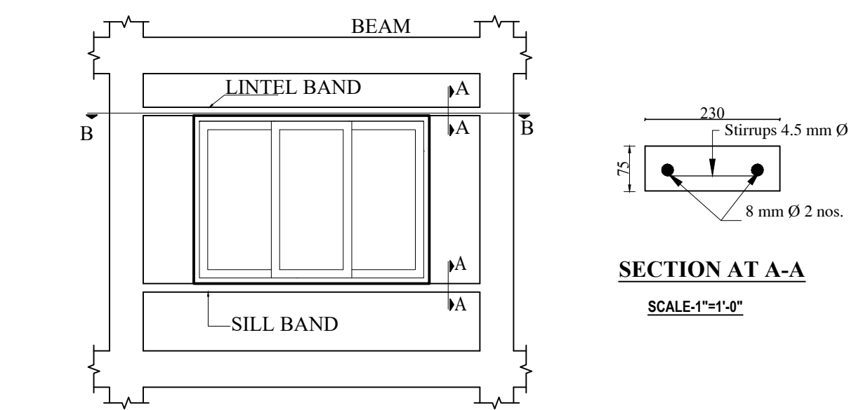
SILL AND LINTEL BAND SCALE-1/4"=1'-0"
