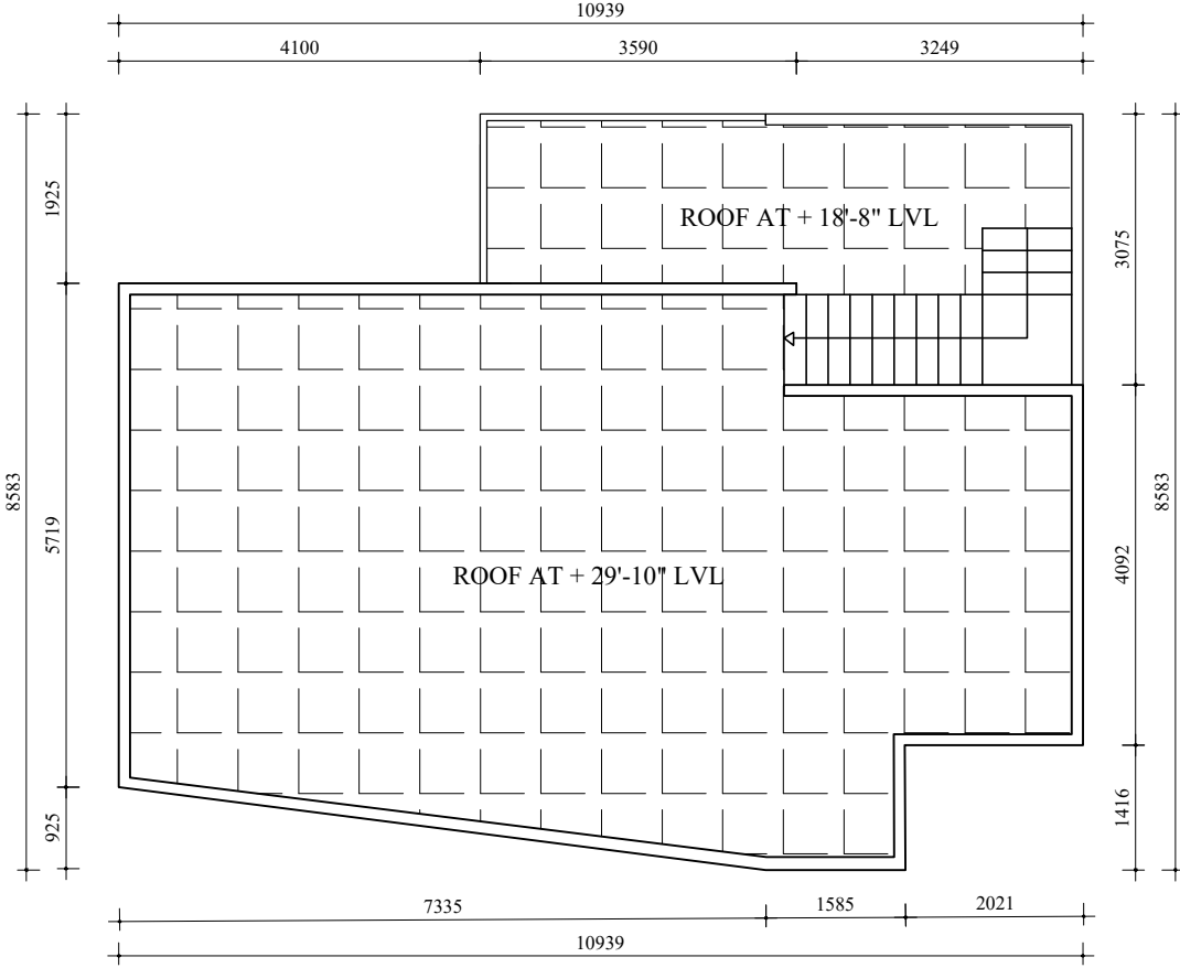
ROOF PLAN
