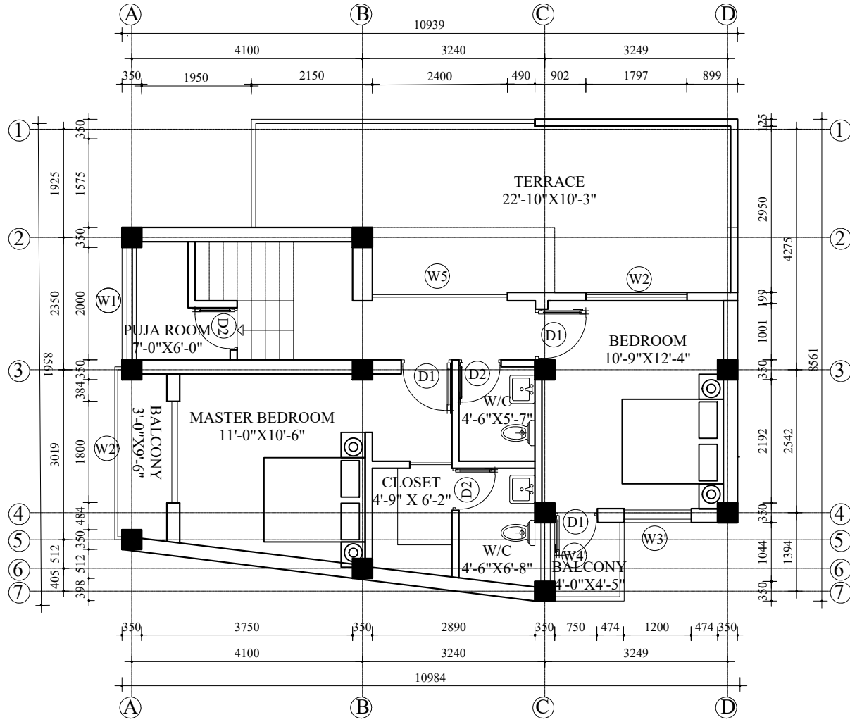
2ND FLOOR PLAN AREA: 635 SQ. FT
