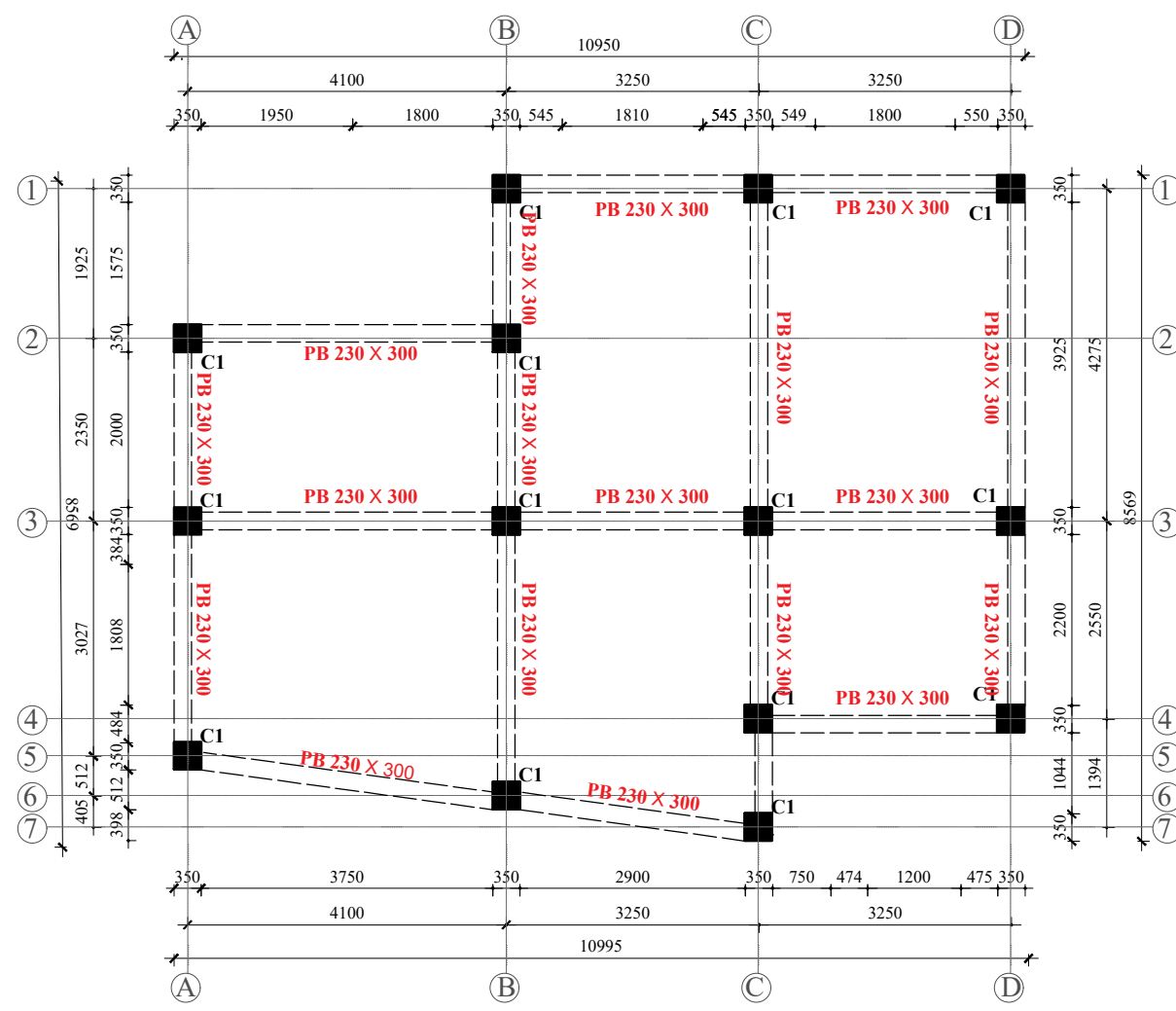
COLUMN & PLINTH BEAM PLAN SCALE :- 1" = 8'-0"
