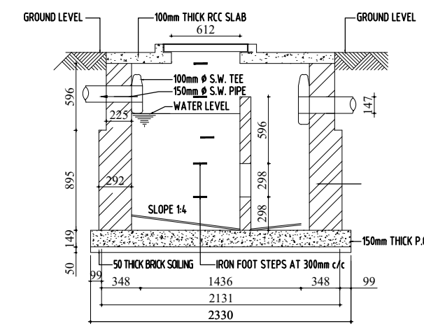
CROSS SECTION OF SEPTIC TANK SCALE :- 1" = 4'-0"
