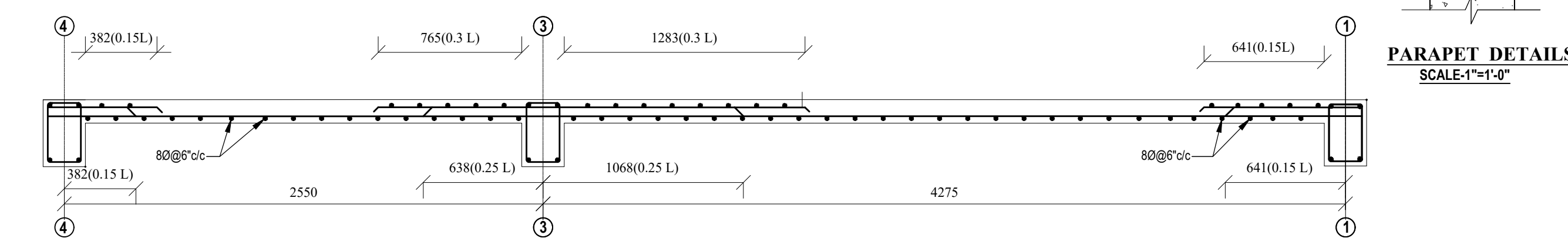
SLAB SECTION AT Y-Y SCALE :- 1/2" = 1'-0"
