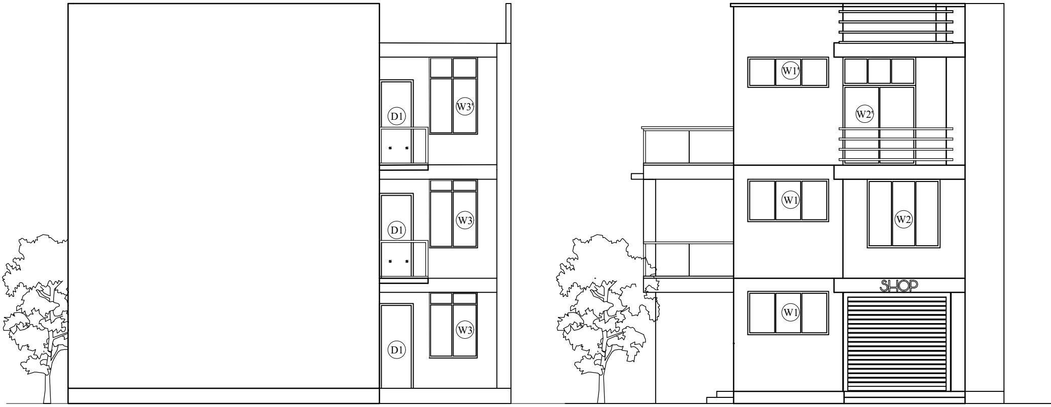
SOUTH ELEVATION
