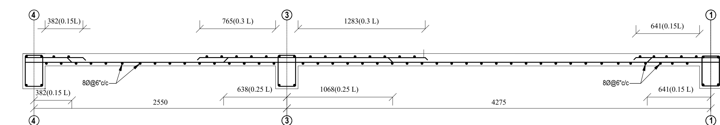
SLAB SECTION AT Y-Y SCALE : 1/2" = 1'-0"
