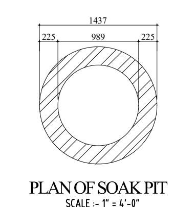
PLAN OF SOAK PIT SCALE :- 1" = 4'-0"
