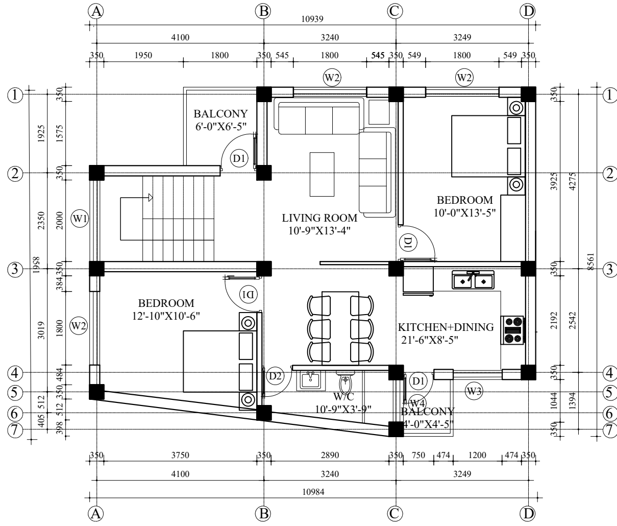
1ST FLOOR PLAN AREA: 900 SQ. FT
