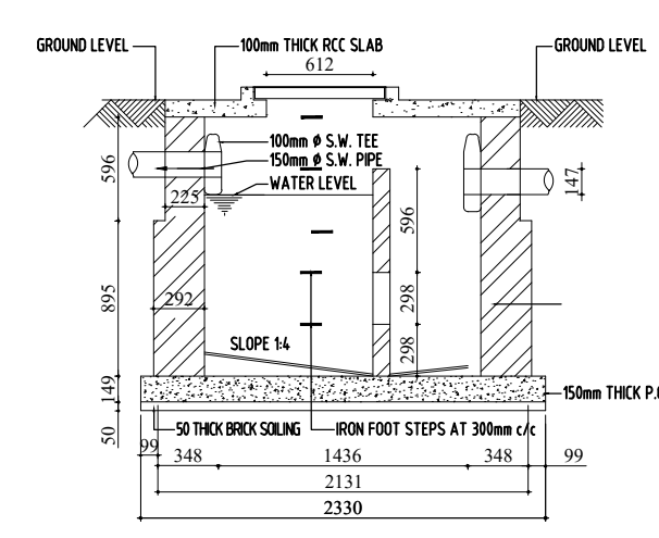
CROSS SECTION OF SEPTIC TANK SCALE :- 1" = 4'-0"
