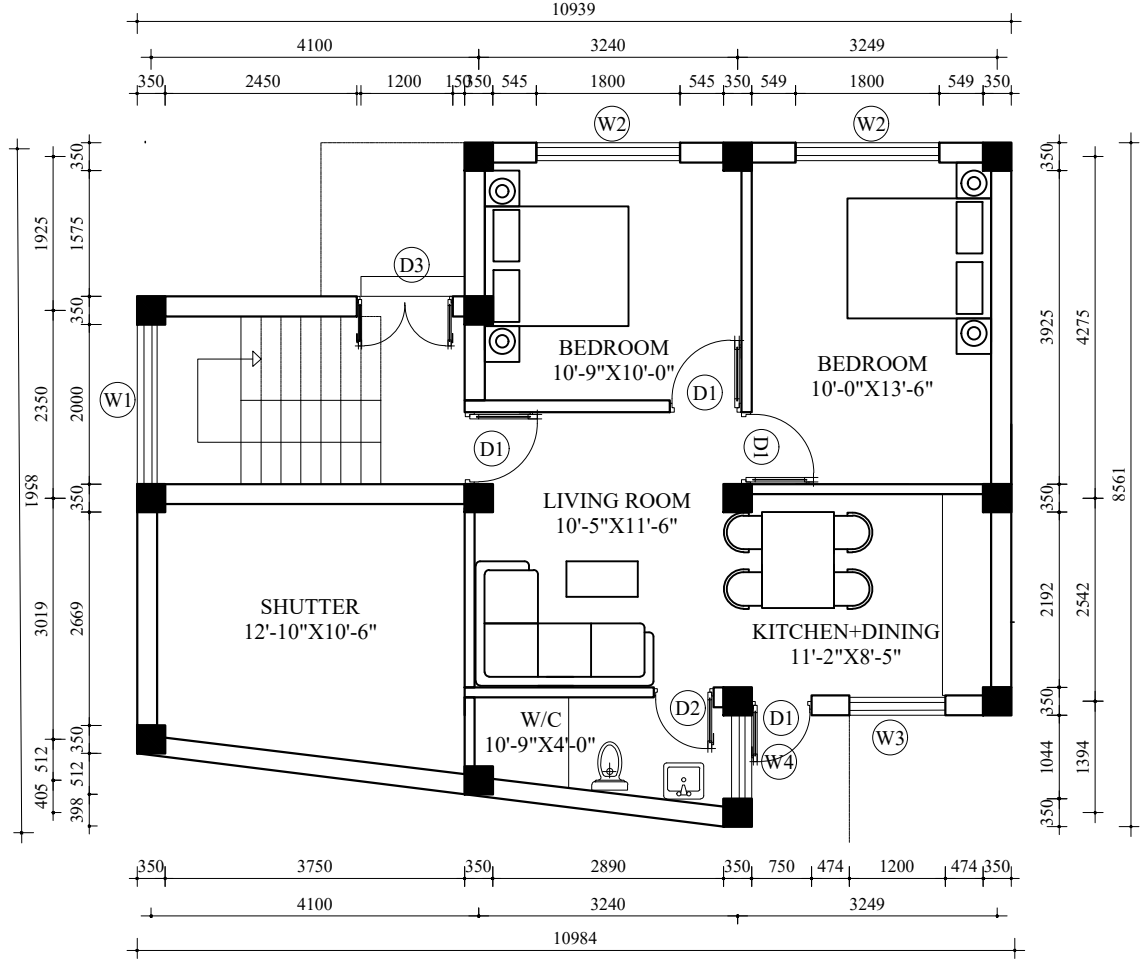
GROUND FLOOR PLAN AREA: 850 SQ. FT
